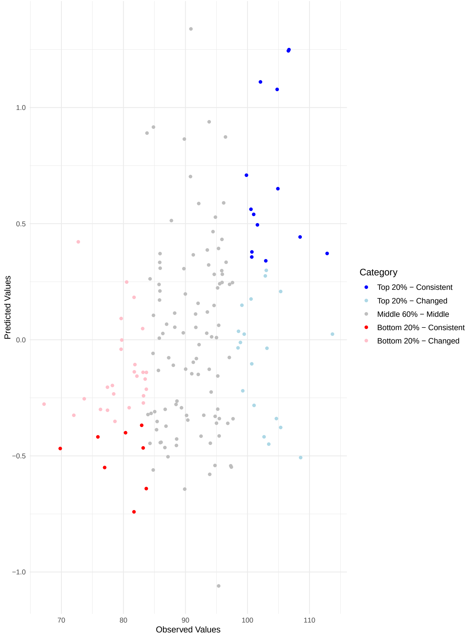
Comparing Predicted and Observed Rankings Across Validation Sets Kendall's Tau: 0.22 | Top 20% Consistency: 26.92% | Bottom 20% Consistency: 13.33%
