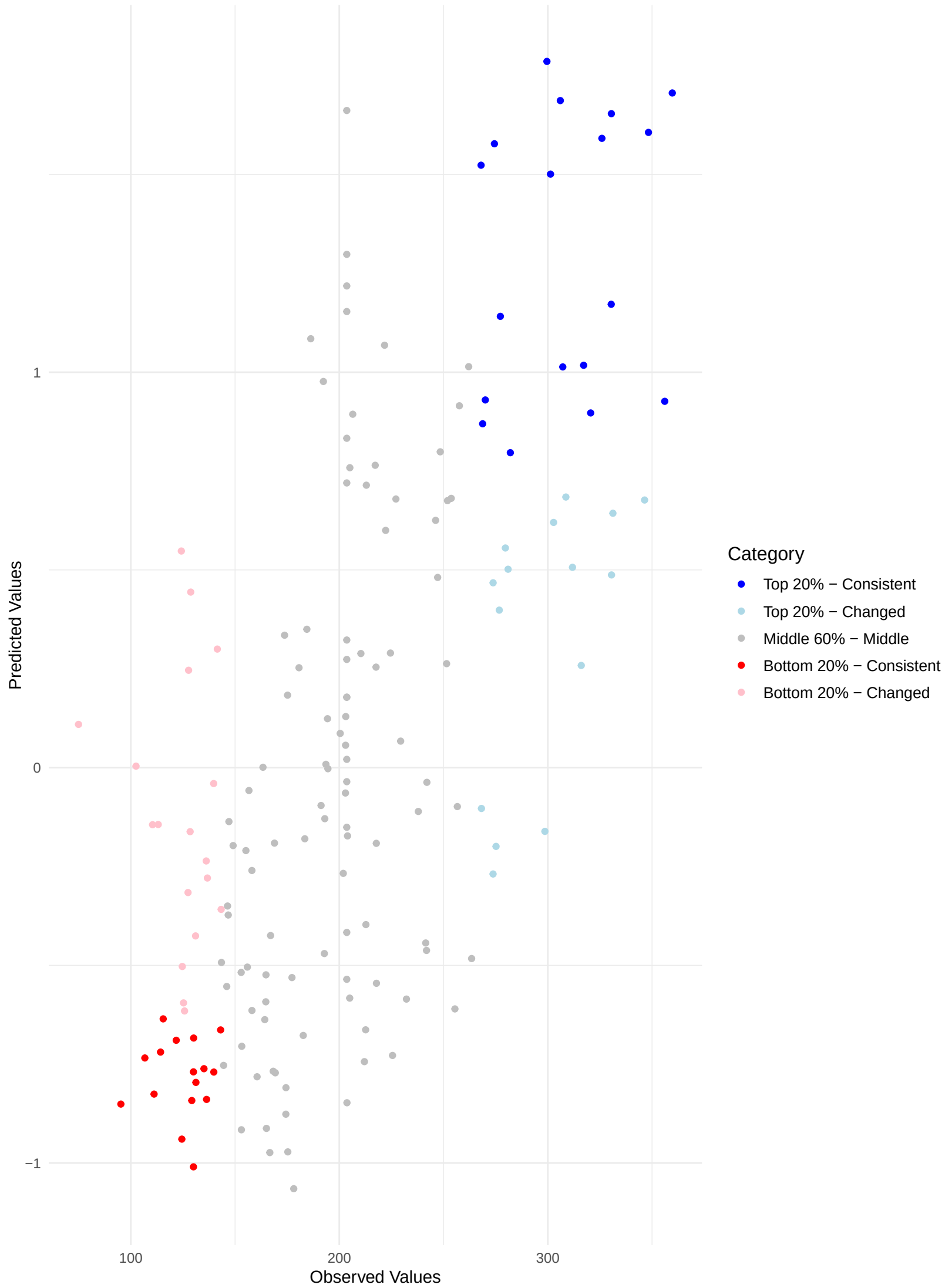
Comparing Predicted and Observed Rankings Across Validation Sets Kendall's Tau: 0.45 | Top 20% Consistency: 37.50% | Bottom 20% Consistency: 30.77%
