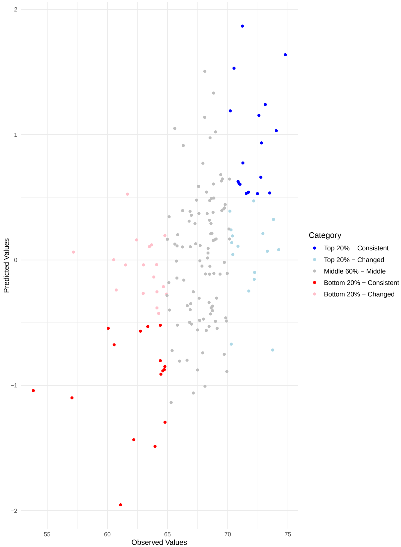
Comparing Predicted and Observed Rankings Across Validation Sets Kendall's Tau: 0.33 | Top 20% Consistency: 34.69% | Bottom 20% Consistency: 30.77%
