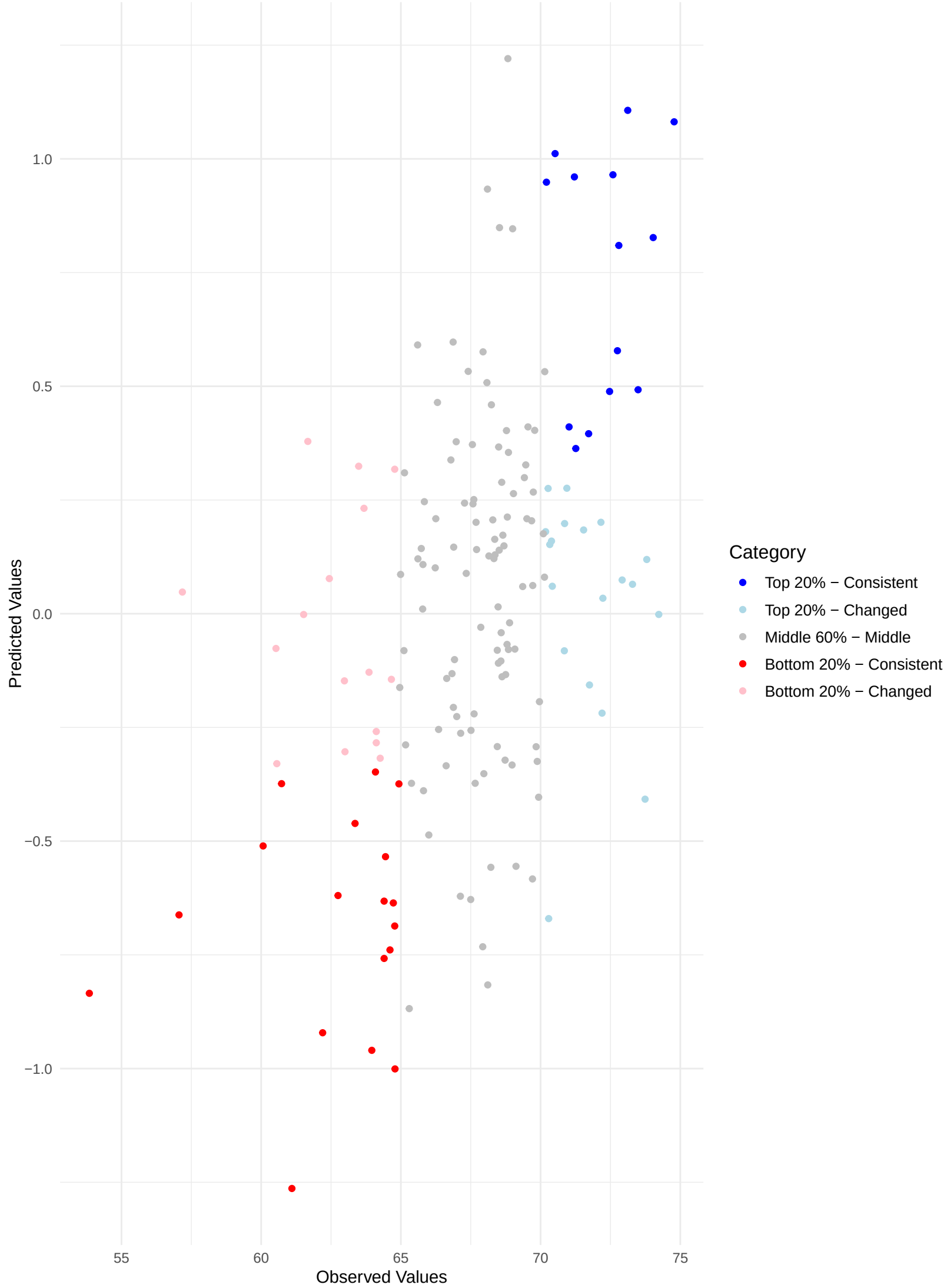
Comparing Predicted and Observed Rankings Across Validation Sets Kendall's Tau: 0.31 | Top 20% Consistency: 26.92% | Bottom 20% Consistency: 36.00%
