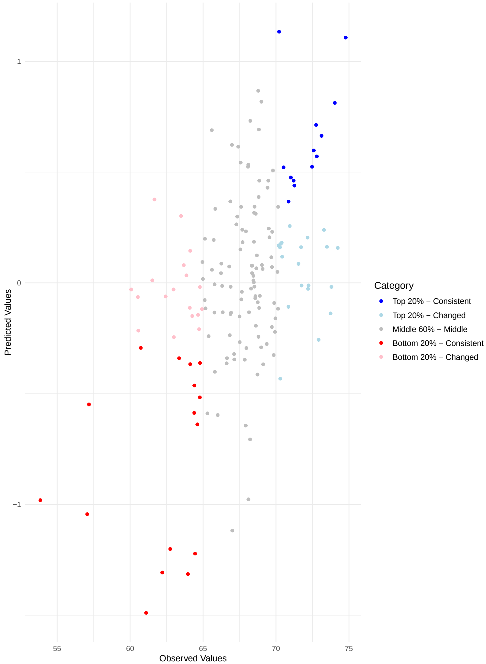
Comparing Predicted and Observed Rankings Across Validation Sets Kendall's Tau: 0.31 | Top 20% Consistency: 24.53% | Bottom 20% Consistency: 30.77%
