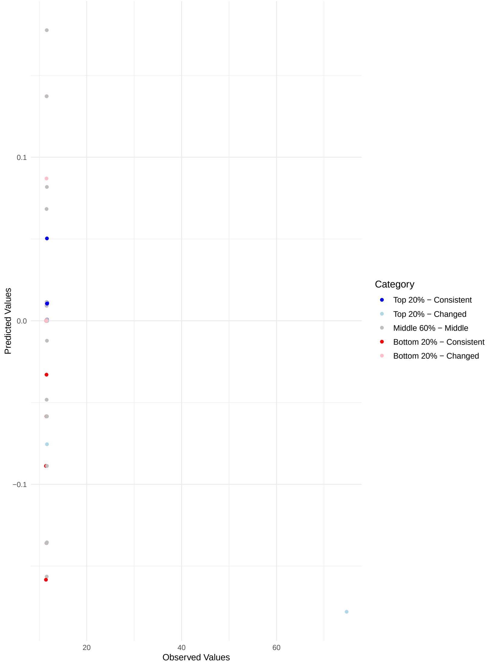
Comparing Predicted and Observed Rankings Across Validation Sets Kendall's Tau: 0.01 | Top 20% Consistency: 12.68% | Bottom 20% Consistency: 15.94%
