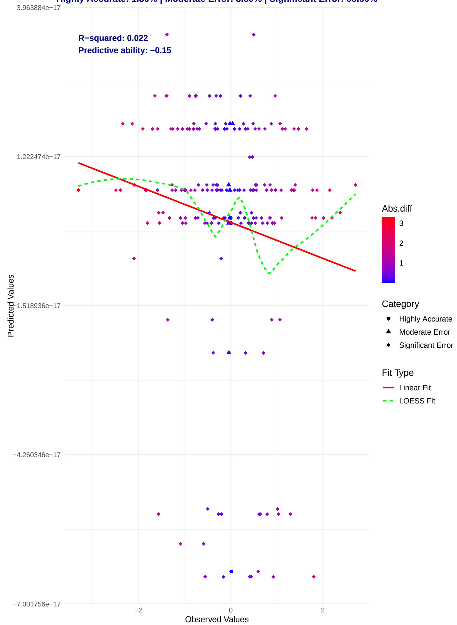
Evaluation of Observed vs Predicted Values with Linear and LOESS Fits Highly Accurate: 1.50% | Moderate Error: 3.50% | Significant Error: 95.00%
