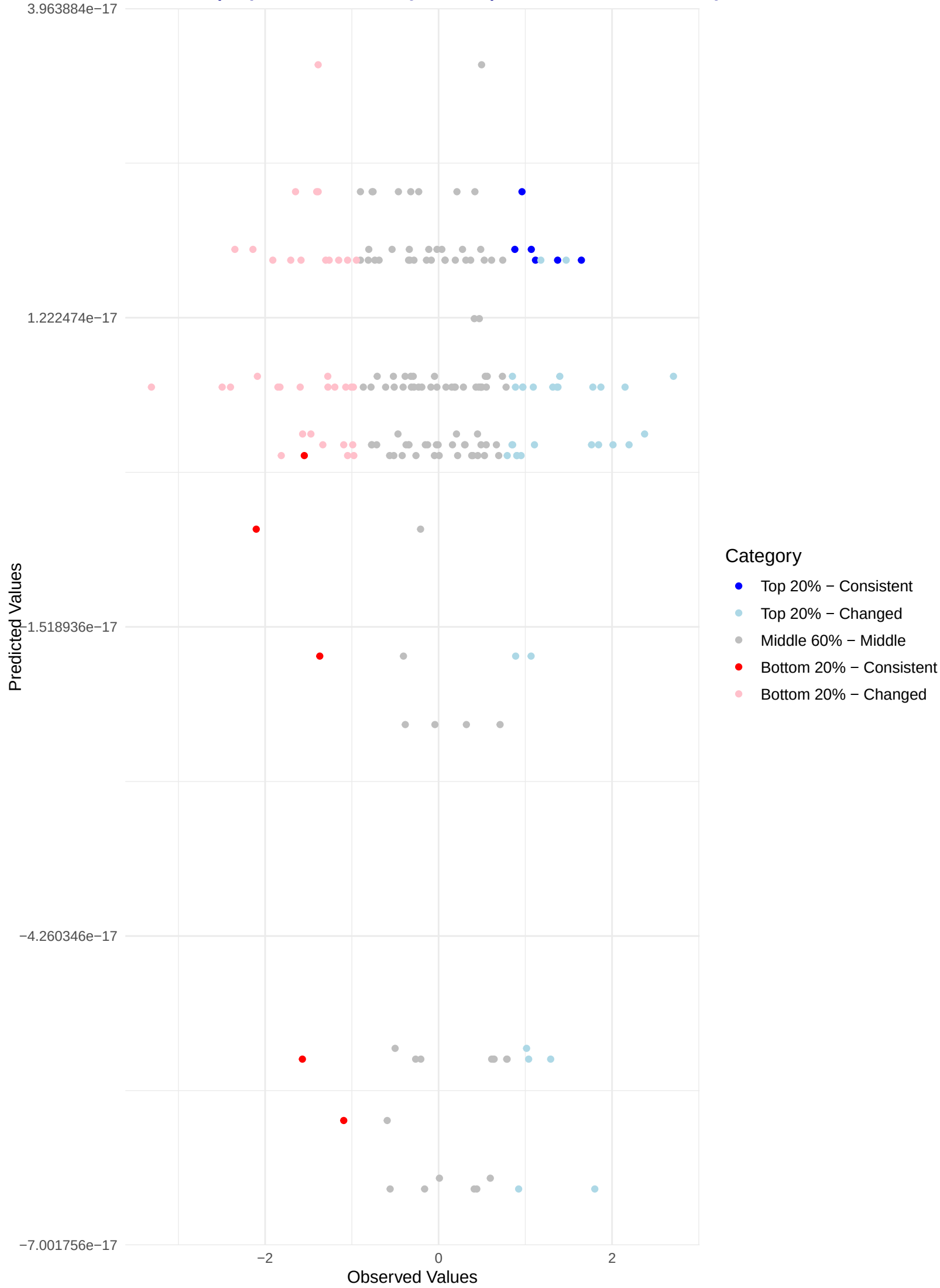
Comparing Predicted and Observed Rankings Across Validation Sets Kendall's Tau: -0.11 | Top 20% Consistency: 8.11% | Bottom 20% Consistency: 6.67%
