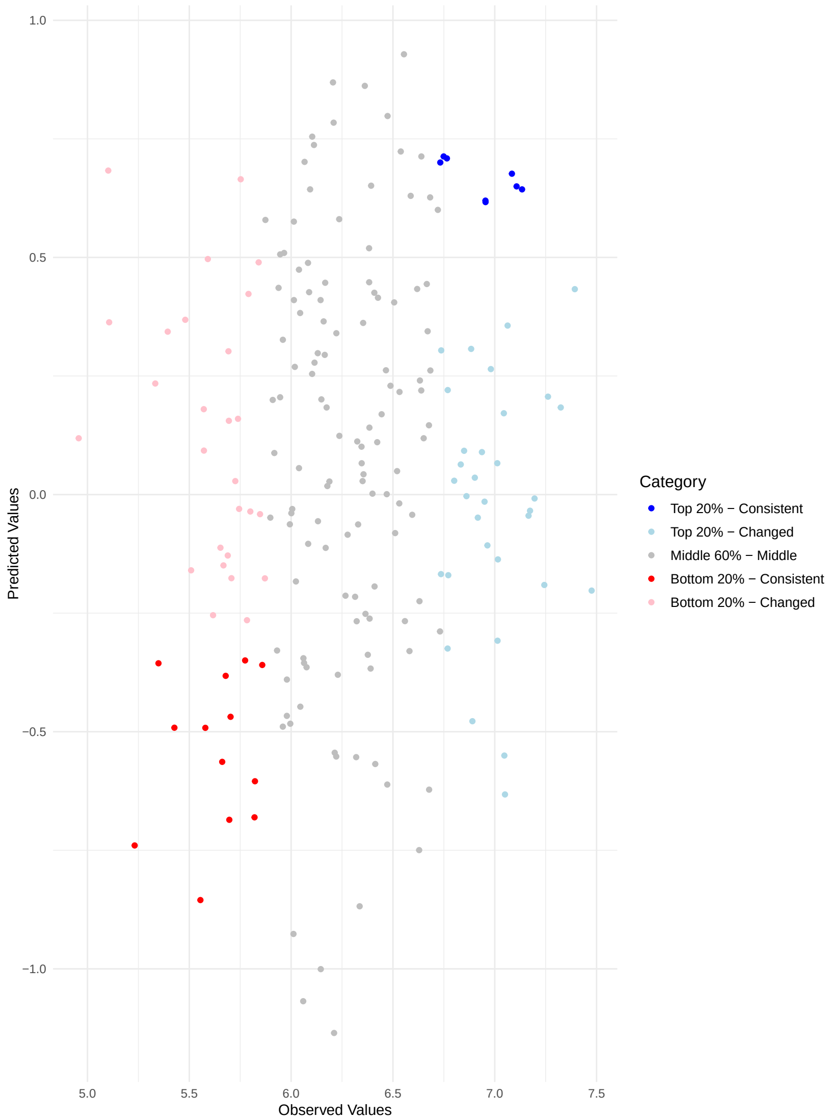
Comparing Predicted and Observed Rankings Across Validation Sets Kendall's Tau: 0.09 | Top 20% Consistency: 11.11% | Bottom 20% Consistency: 19.40%
