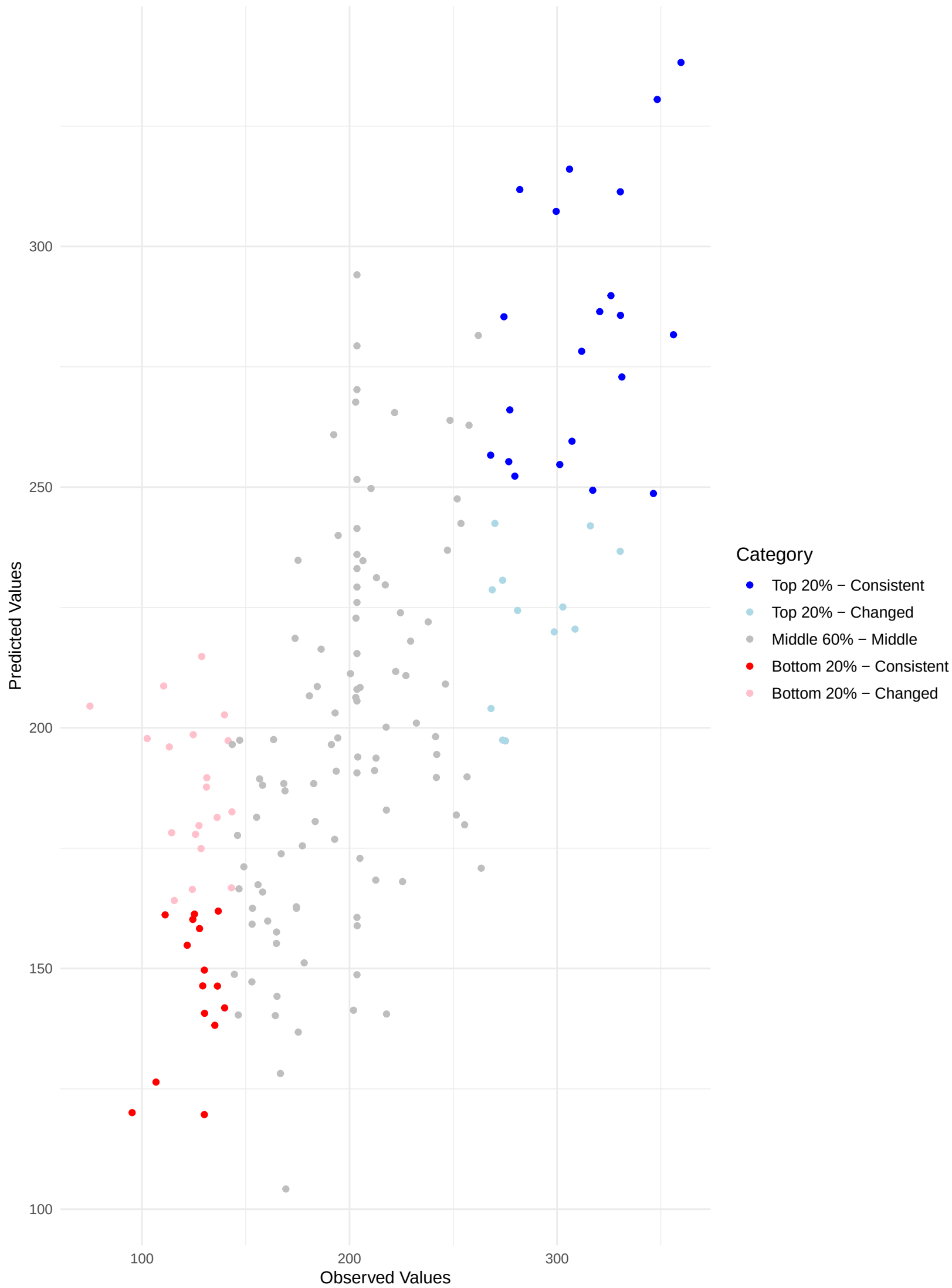
Comparing Predicted and Observed Rankings Across Validation Sets Kendall's Tau: 0.49 | Top 20% Consistency: 46.67% | Bottom 20% Consistency: 28.30%
