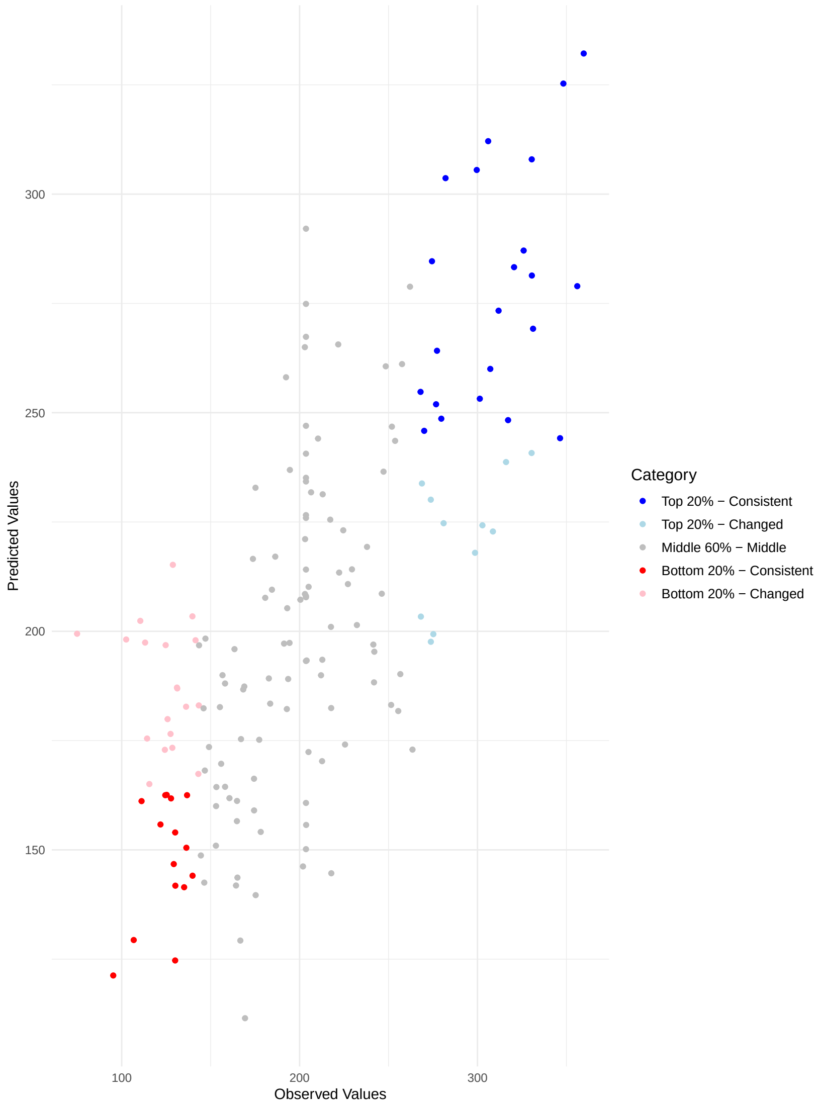
Comparing Predicted and Observed Rankings Across Validation Sets Kendall's Tau: 0.50 | Top 20% Consistency: 50.00% | Bottom 20% Consistency: 28.30%
