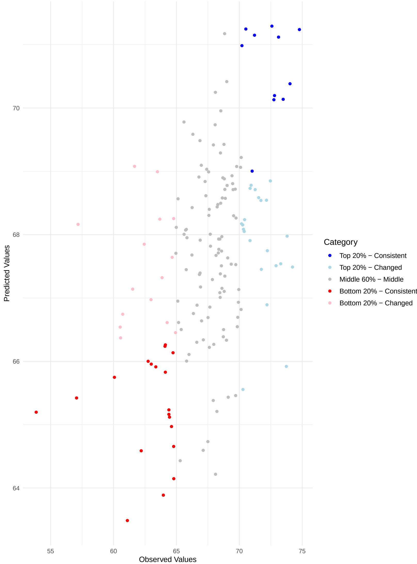
Comparing Predicted and Observed Rankings Across Validation Sets Kendall's Tau: 0.32 | Top 20% Consistency: 20.00% | Bottom 20% Consistency: 38.78%
