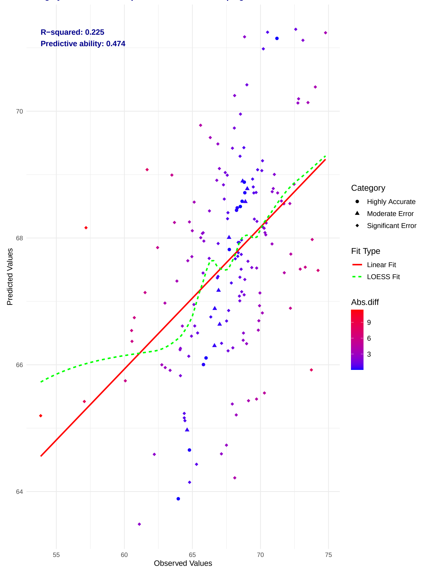
Evaluation of Observed vs Predicted Values with Linear and LOESS Fits Highly Accurate: 7.14% | Moderate Error: 5.36% | Significant Error: 87.50%
