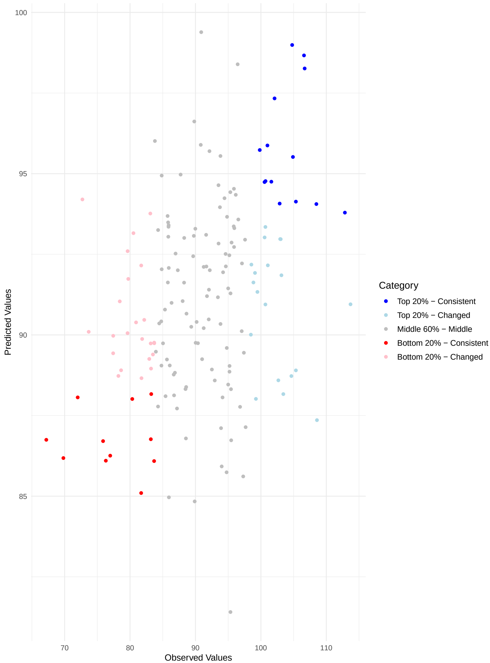
Comparing Predicted and Observed Rankings Across Validation Sets Kendall's Tau: 0.22 | Top 20% Consistency: 26.92% | Bottom 20% Consistency: 19.30%
