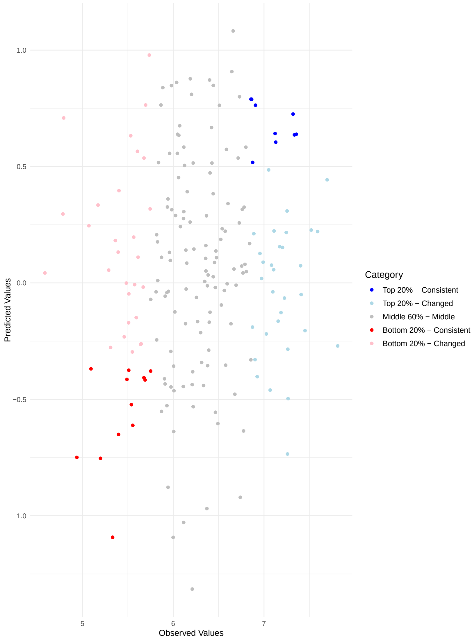
Comparing Predicted and Observed Rankings Across Validation Sets Kendall's Tau: 0.09 | Top 20% Consistency: 12.68% | Bottom 20% Consistency: 17.65%
