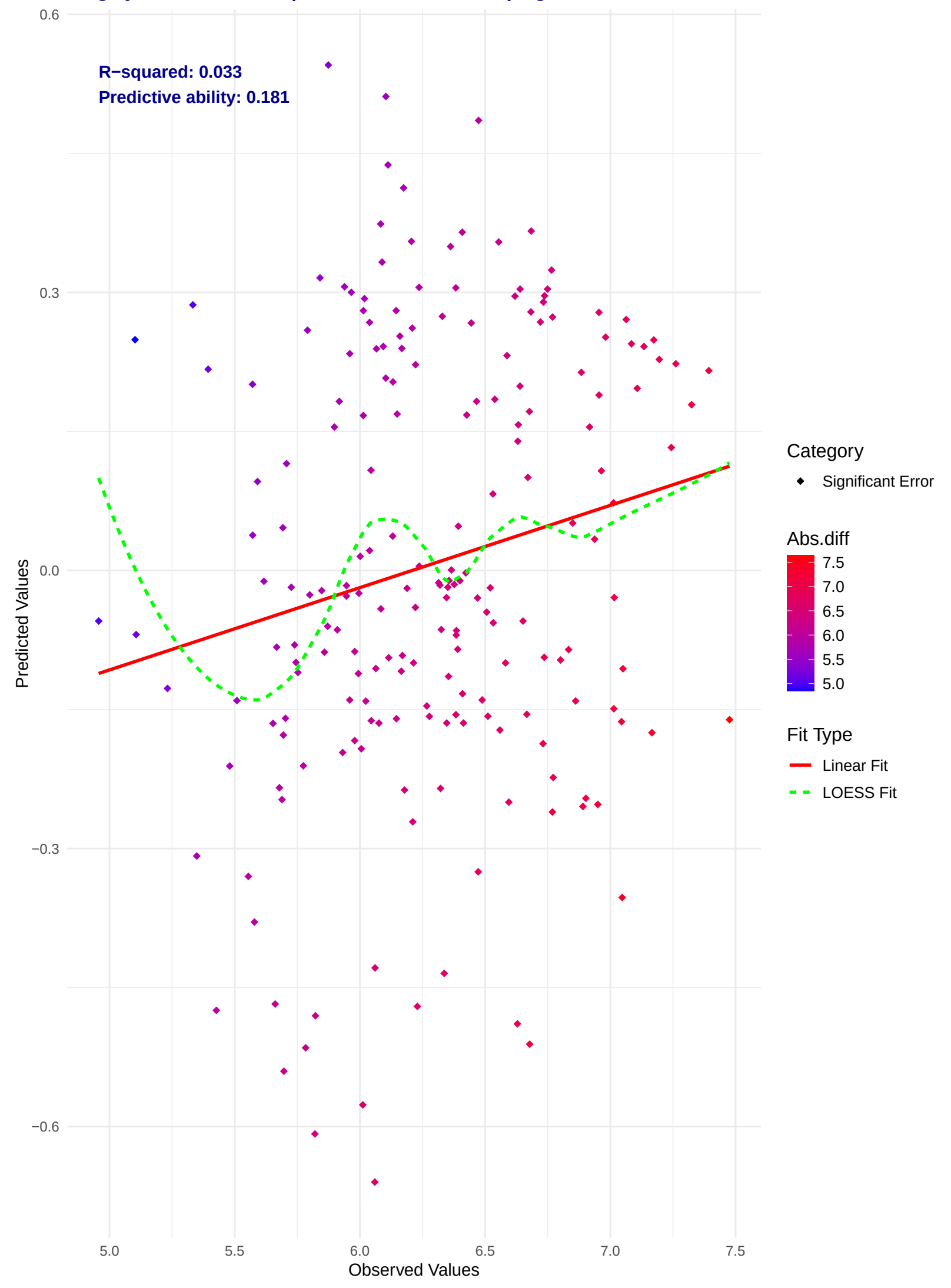
Evaluation of Observed vs Predicted Values with Linear and LOESS Fits Highly Accurate: 0.00% | Moderate Error: 0.00% | Significant Error: 100.00%
