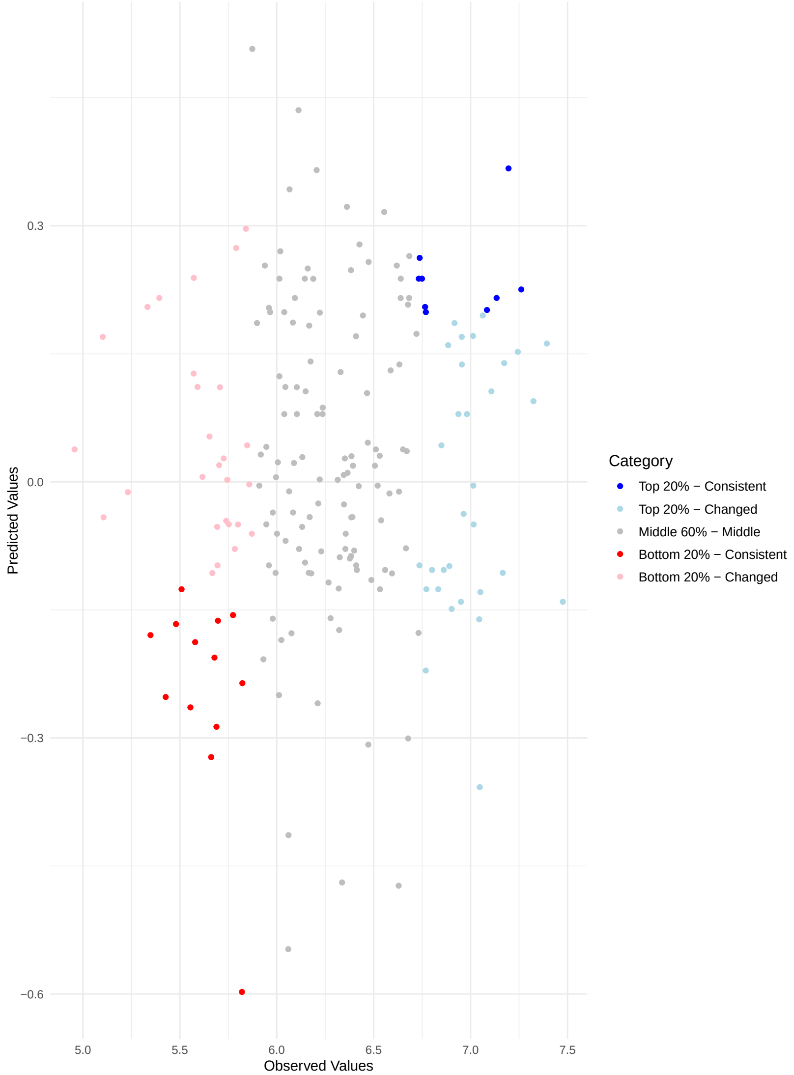
Comparing Predicted and Observed Rankings Across Validation Sets Kendall's Tau: 0.08 | Top 20% Consistency: 12.68% | Bottom 20% Consistency: 19.40%
