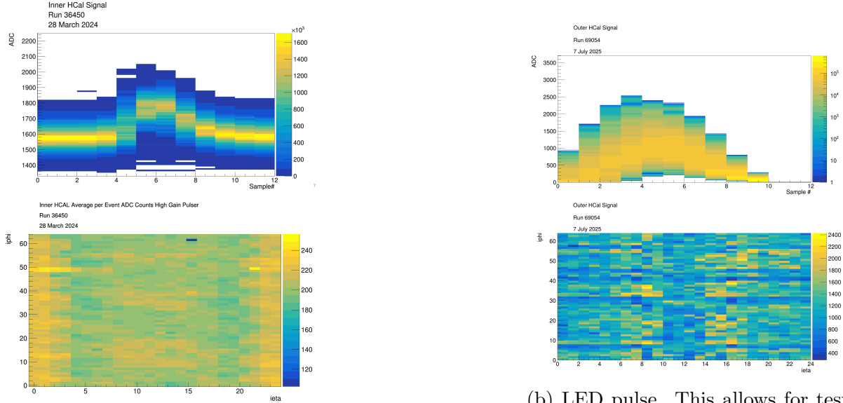
(b) LED pulse. This allows for testing of the full readback system and light response
