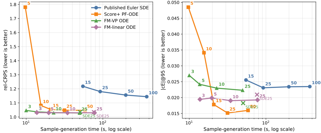
Figure 1: Sampler cost tradeoff after tuning, averaged over the same ten UCI datasets and folds 1–5. Points are eval-only sampler changes from the tuned configurations; labels show solver steps, and SDE25 marks the 25-step stochastic FM sampler. rel-CRPS is normalized by the best sampler-cost row on each dataset.
