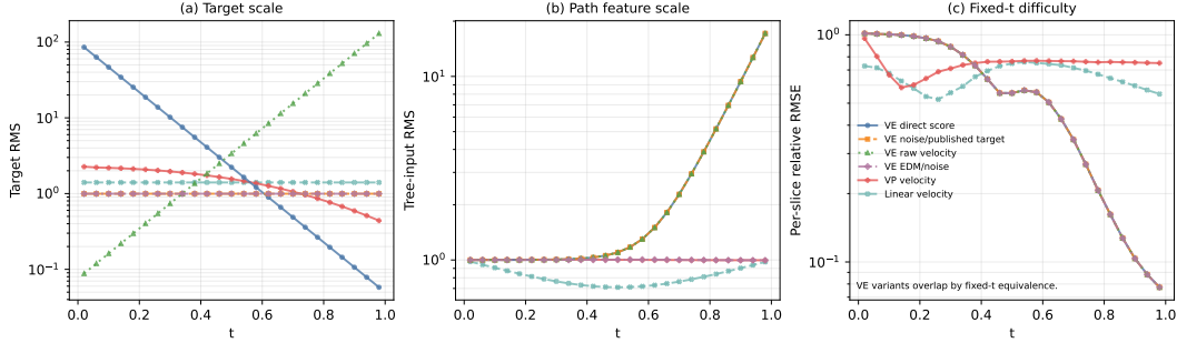
Figure 2: Toy preconditioning diagnostic on a one-dimensional heteroscedastic mixture, generated by pixi run toy-geometry . Panel (a) shows that direct VE score prediction and raw VE-FM have target scales that vary by orders of magnitude across t , whereas the published-style VE noise target, EDM/noise prediction, and linear velocity have unit target scale. Panel (b) separates target scaling from input geometry: the published-style VE target is stable but the tree input y_t = y_0 + \sigma z still expands strongly, while EDM rescales the input and VP-FM keeps the path feature near standardized scale. Panel (c) fits a fresh LightGBM at each fixed t ; the VE curves overlap up to numerical noise, confirming that the score/velocity distinction is not intrinsic fixed- t smoothness but cross- t conditioning.
