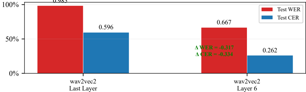
Layer Ablation: wav2vec 2.0 Last vs Layer 6
