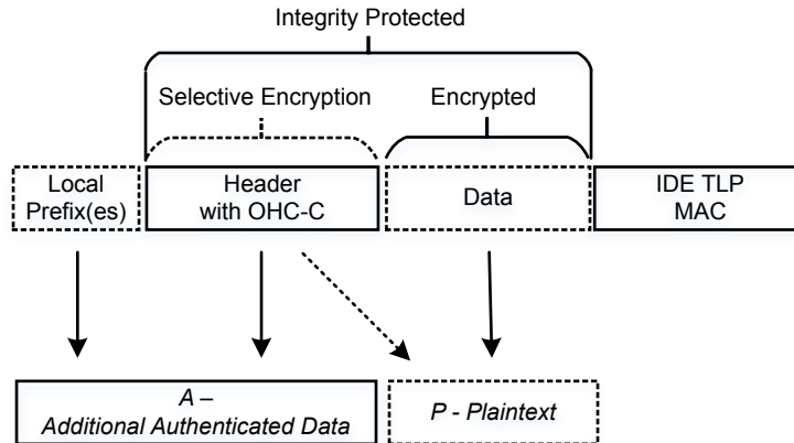
Figure 6-68 IDE TLP – Example of IDE TLP for a Selective IDE Stream without Aggregation (Flit Mode)
