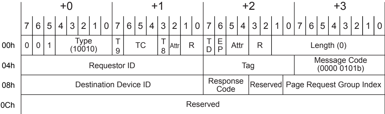
Figure 10-27 PRG Response Message - Non-Flit Mode
