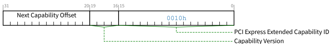
Figure 9-11 SR-IOV Extended Capability Header
