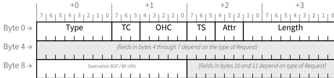
Figure 2-24 ID Routing with 3 DW Header - Flit Mode
