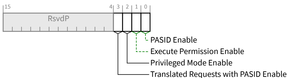
§ Figure 7-188 PASID Control Register
