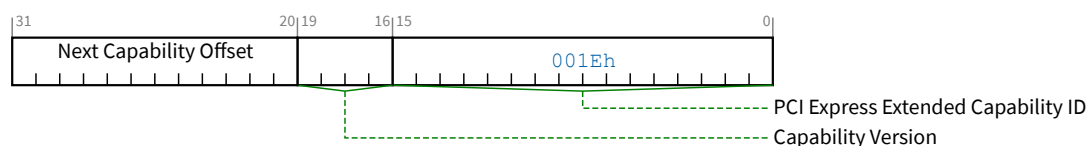
Figure 7-147 L1 PM Substates Extended Capability Header
