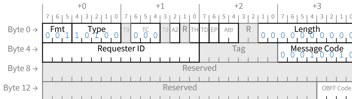
Figure 2-59 OBFF Message - Non-Flit Mode
