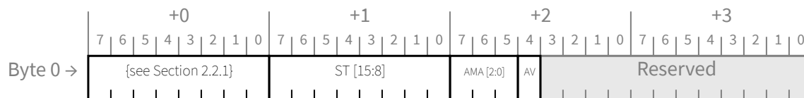
Figure 2-34 TPH TLP Prefix
