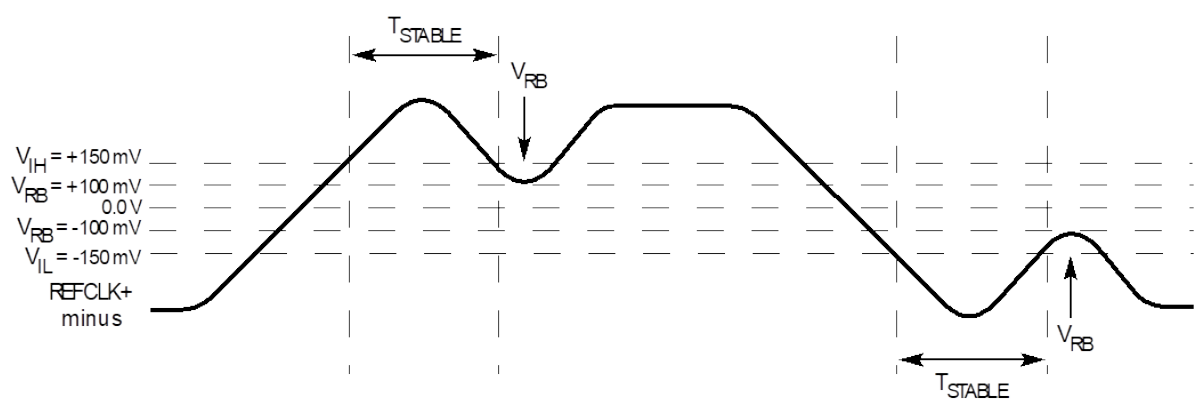
Figure 8-86 Differential Measurement Points for Ringback
