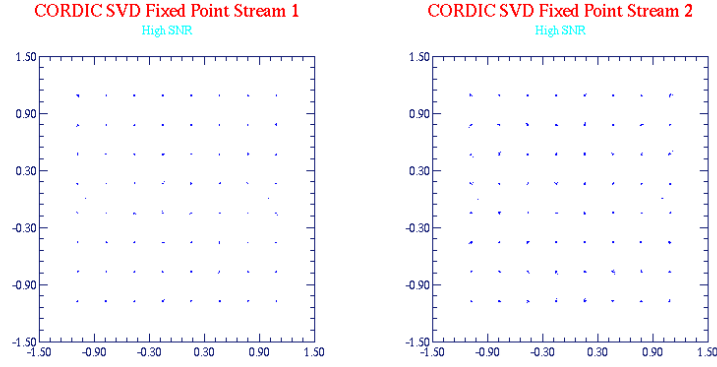
Figure 7: 2x2 Beam Forming MIMO OFDM 64 QAM Constellations for Each Stream CORDIC Fixed Point 2x2 SVD , High SNR
