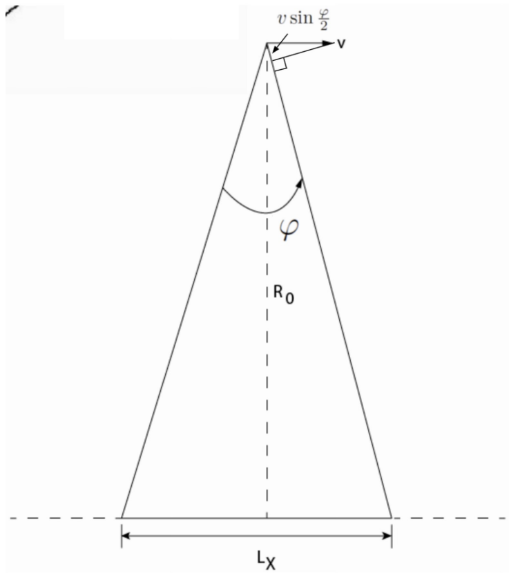
Figure 6: Viewing Geometry Azimuth Plane
