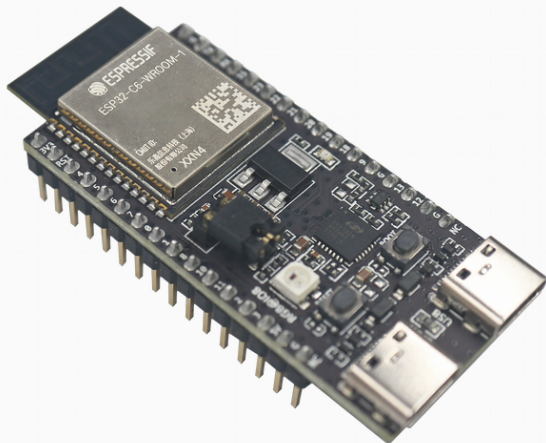
ESP32-C6-DevKitC-1
