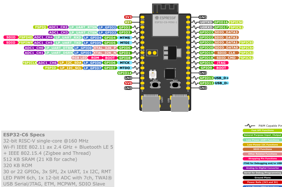
Fig. 4: ESP32-C6-DevKitM-1 Pin Layout (click to enlarge)
