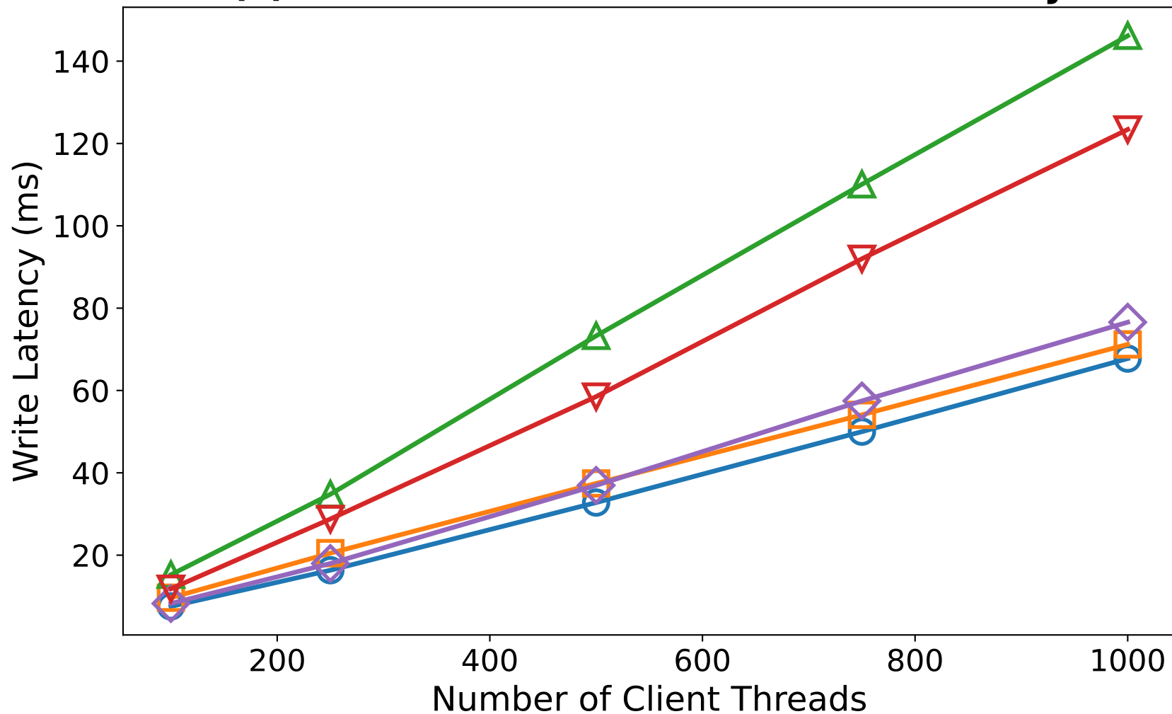
(c) Number of Clients vs. Write Latency
