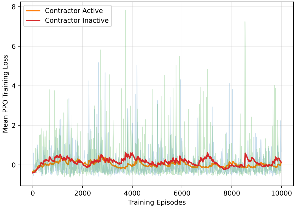
Optimization Stability
