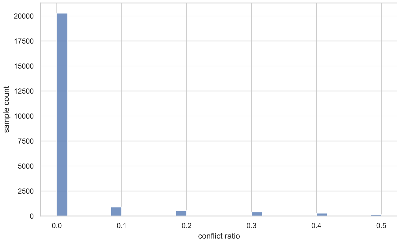
Per-Sample Conflict Ratio
