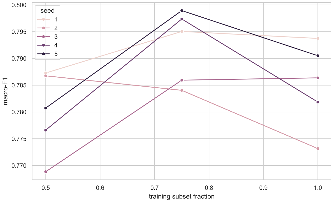
Macro-F1 Across Training Subsets
