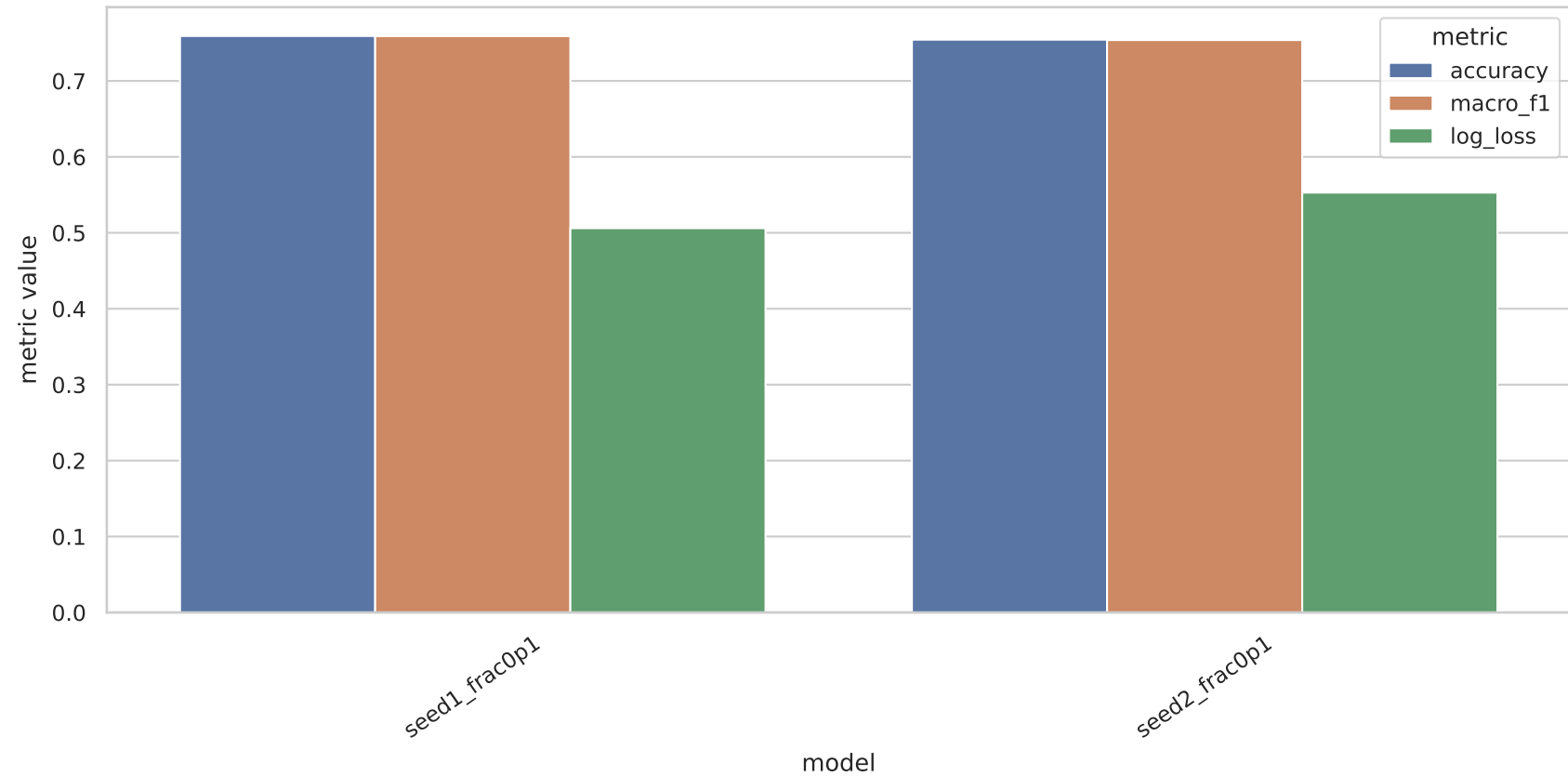
Model-Level Performance
