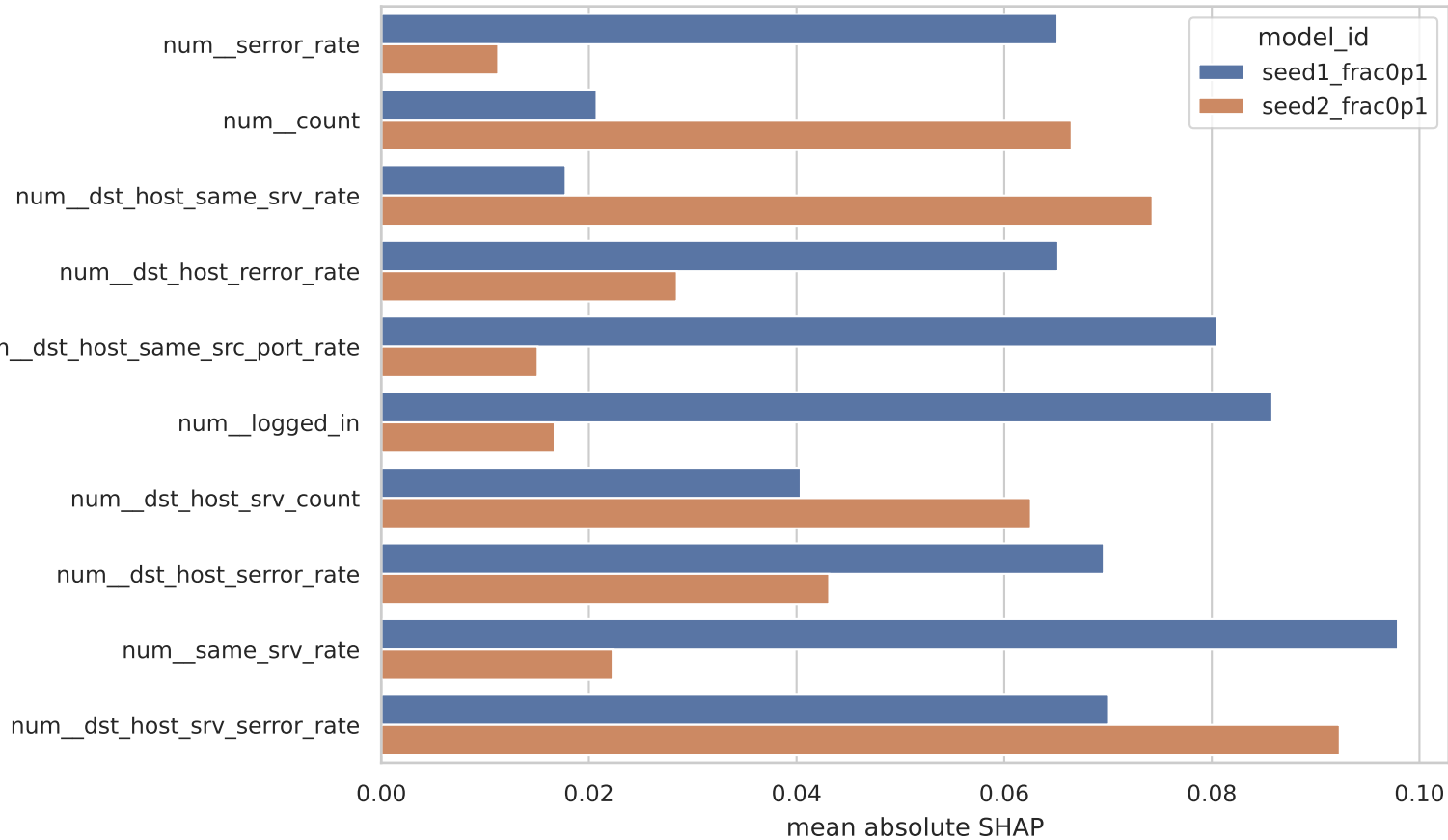
Top SHAP Features: attack
