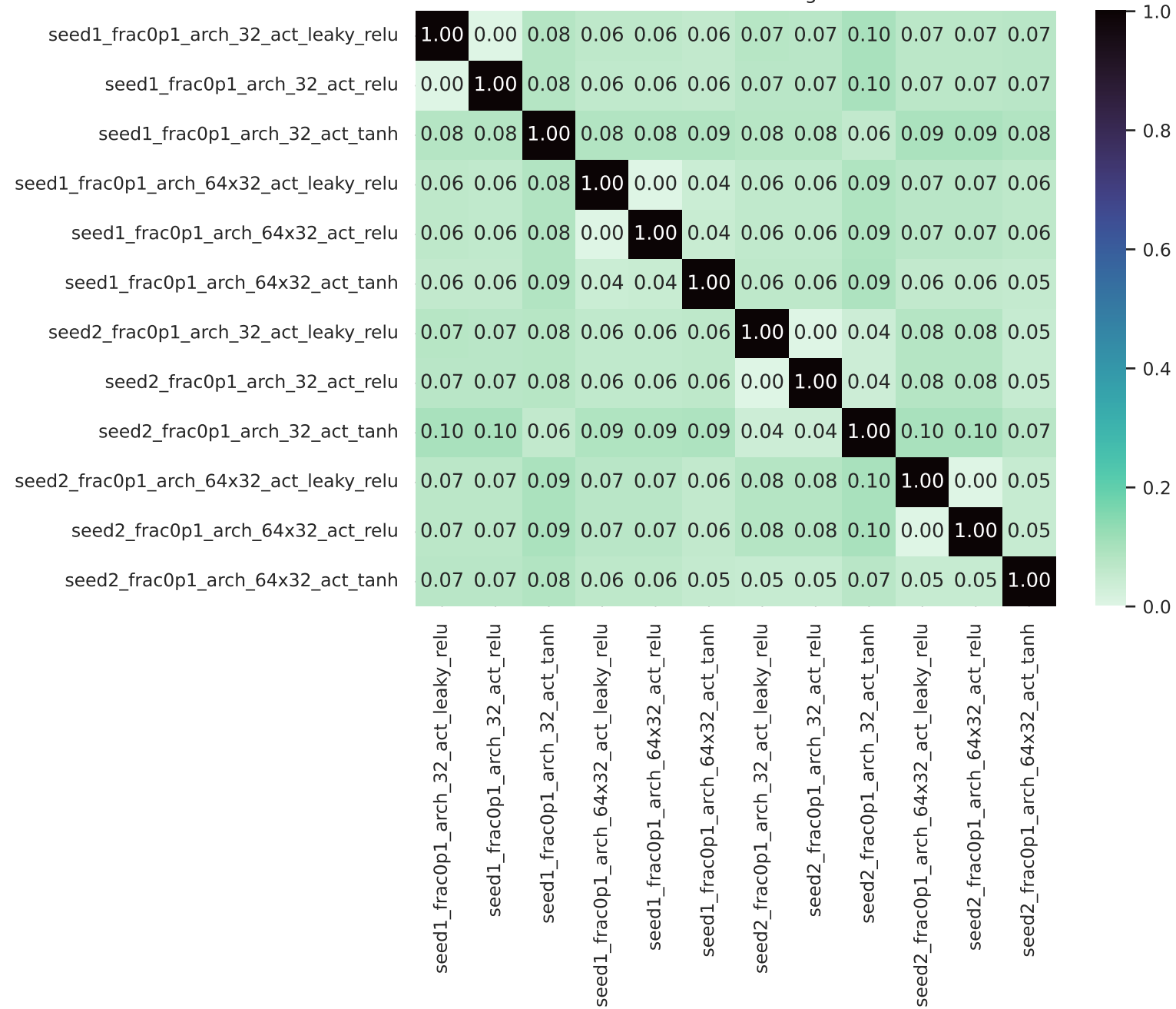
Pairwise Prediction Disagreement
