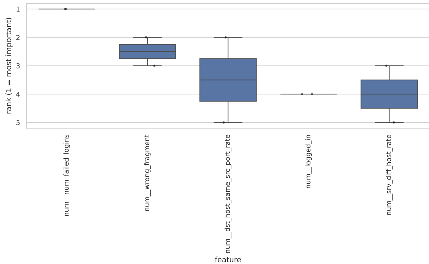
attack: Distribution of Feature Rankings
