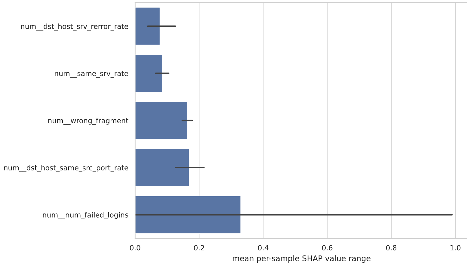
SHAP Value Range Across Models: attack
