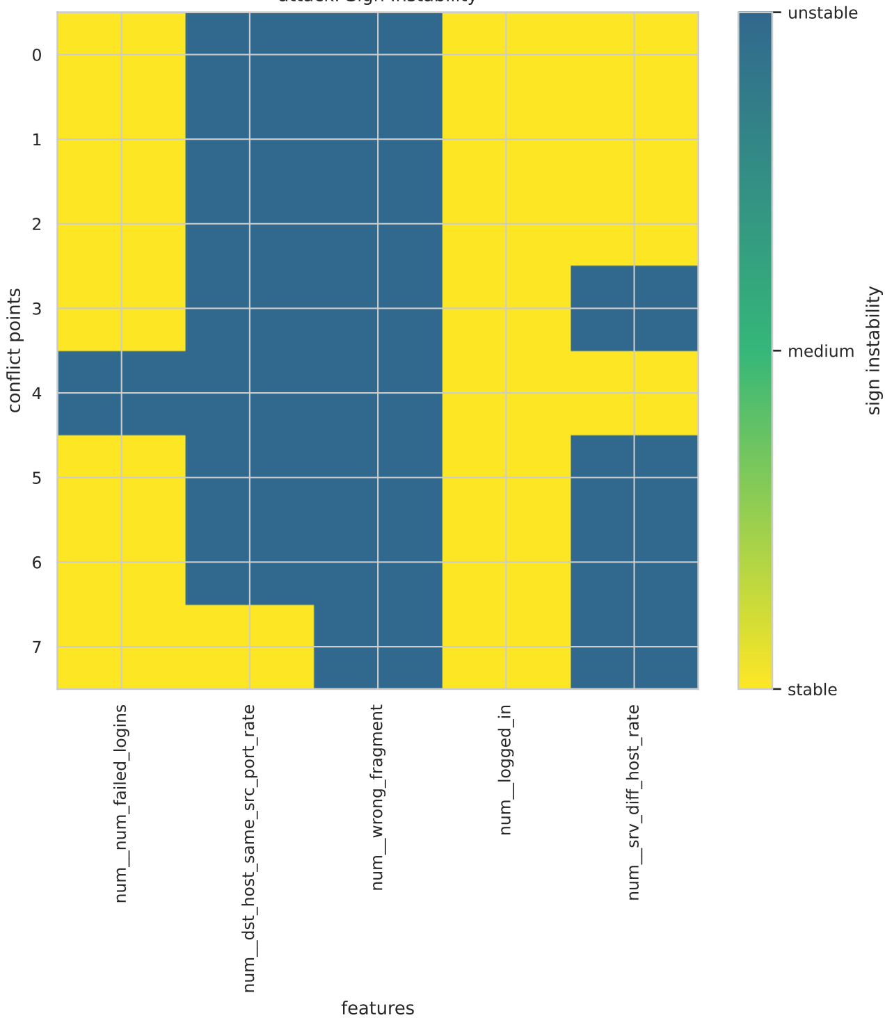
attack: Sign Instability
