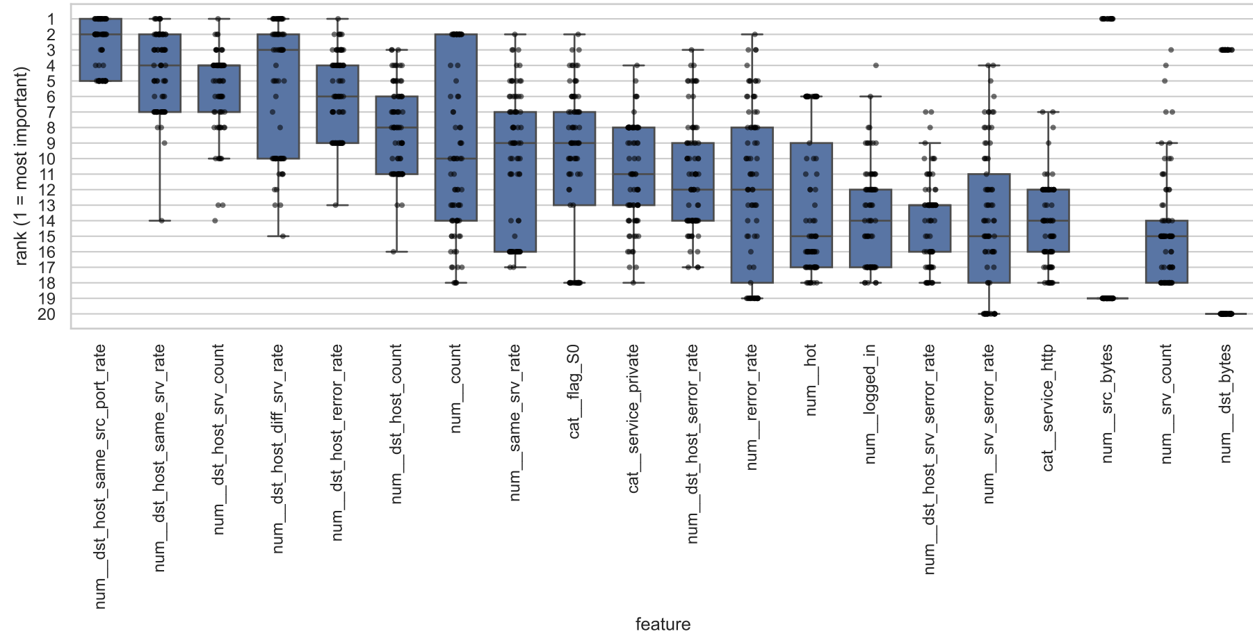
attack: Distribution of Feature Rankings
