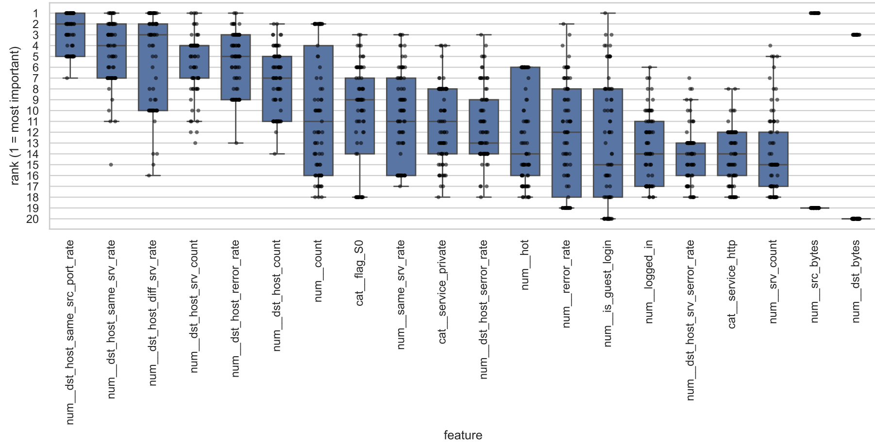
normal: Distribution of Feature Rankings
