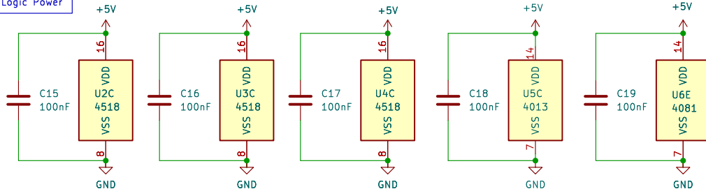
4000 Logic Power
