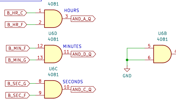
Decoding Logic
