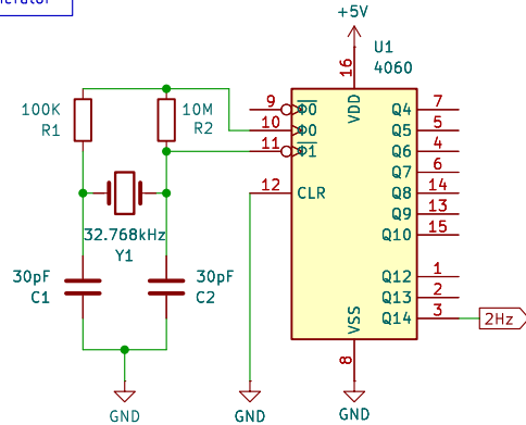
Clock Generator
