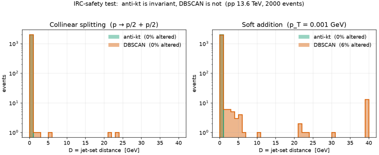
Figure 1: Jet-set distance D [Eq. (4)] under a collinear splitting (left) and a soft addition (right), for anti- k_t (green) and physical (y, \phi) DBSCAN (orange), over 2000 events. anti- k_t is a delta function at D = 0 ; DBSCAN develops a tail, most severely in the infrared.
