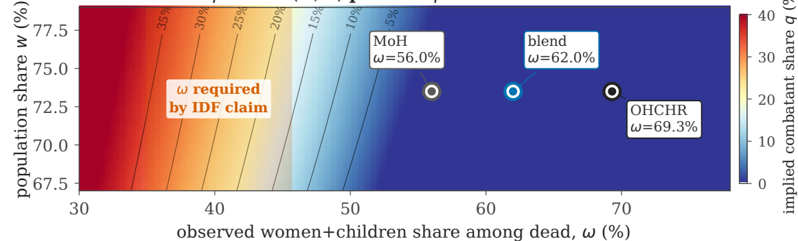
A. Identified q on the (\omega, w) plane at \bar{\mu} = 2.5
