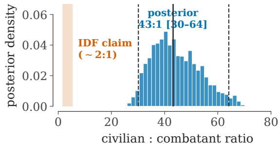
E. Civilian-to-combatant ratio
