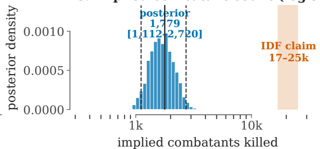
C. Implied combatant count (log scale)
