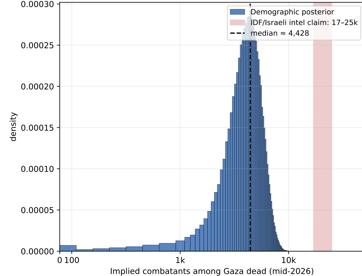
(3) Implied combatants vs IDF/Israeli intel claim
