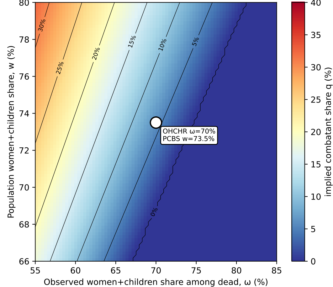
(2) Sensitivity: q = 1 - \omega / w_{\text{civ}} (black contours = q in %)
