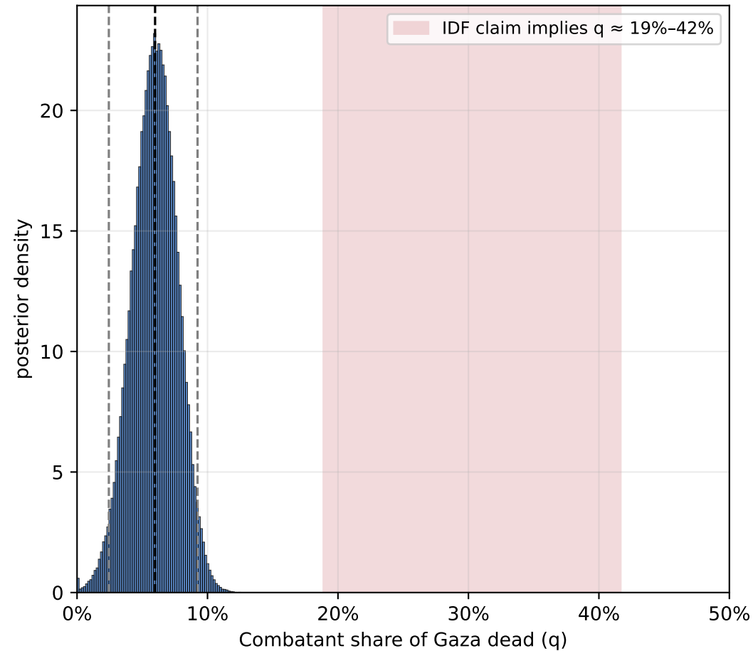
(1) Posterior on q median 6.0%, 95% CI [2.4%, 9.2%]
