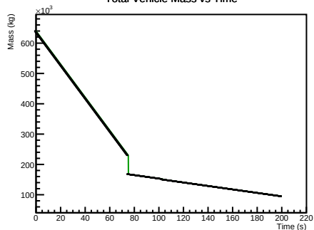
Total Vehicle Mass vs Time
