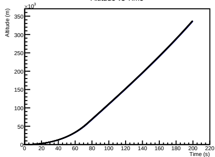
Altitude vs Time
