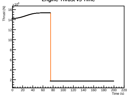
Engine Thrust vs Time
