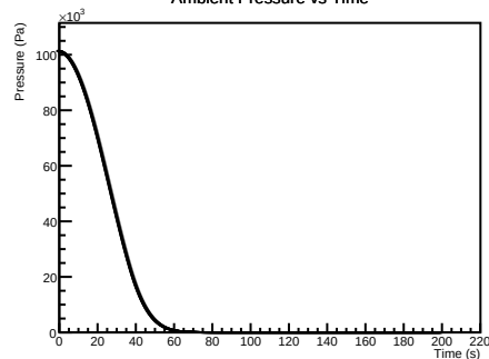
Ambient Pressure vs Time
