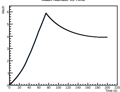
Mach Number vs Time
