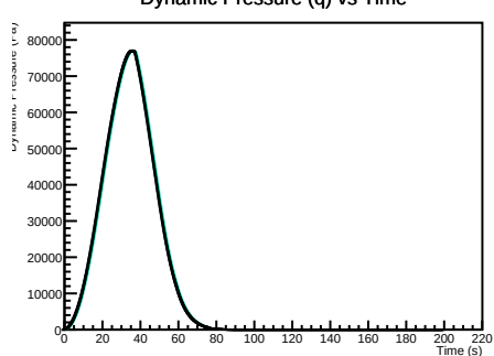
Dynamic Pressure (q) vs Time
