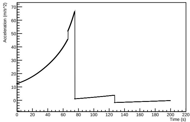
Acceleration vs Time
