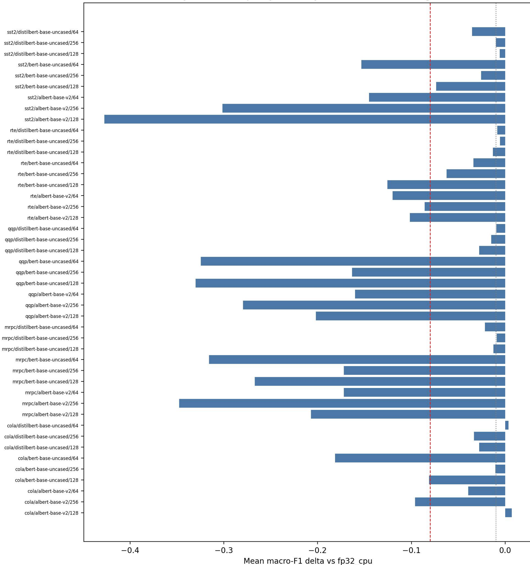
Dynamic INT8 quality deltas by dataset/backbone/budget
