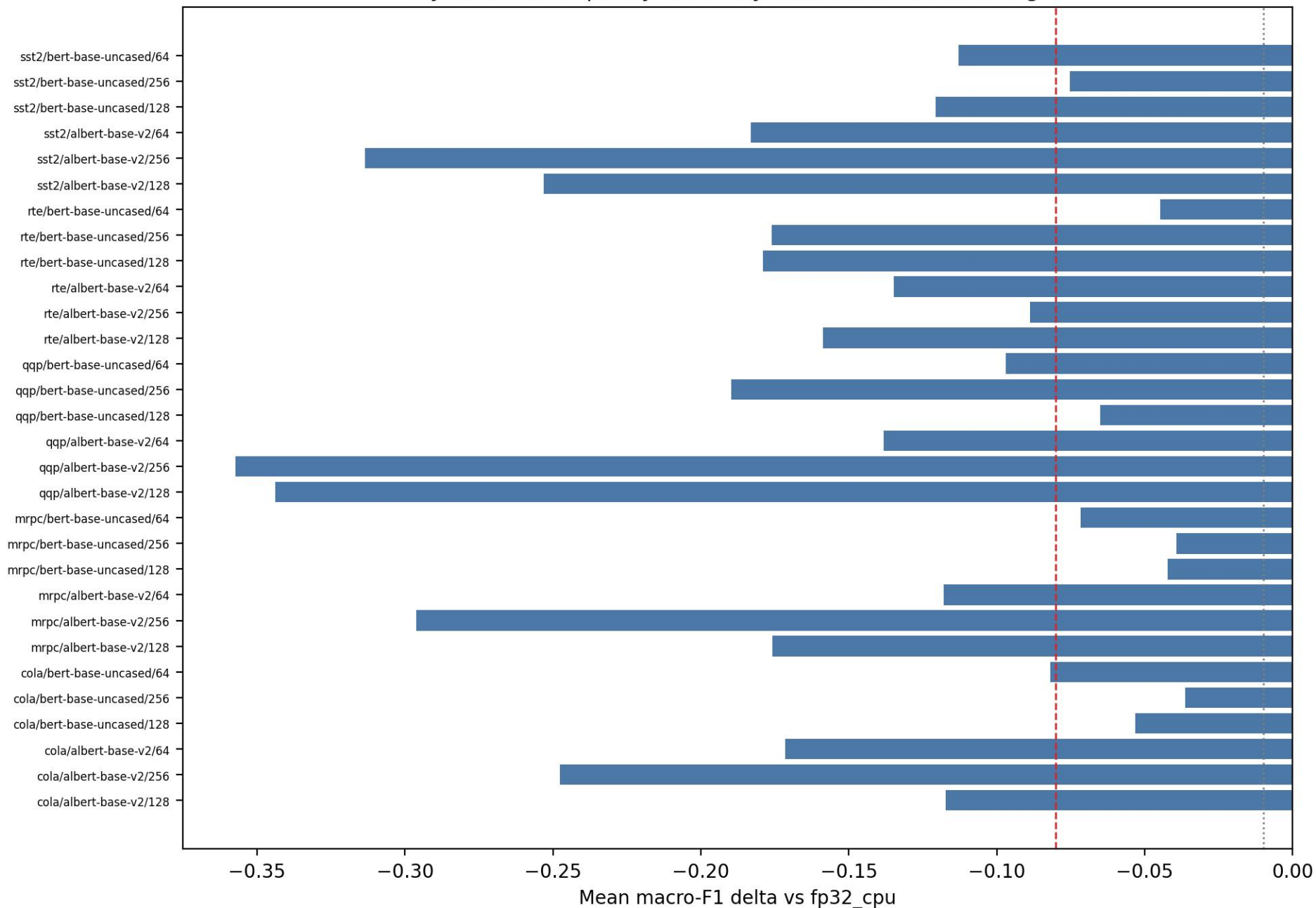
Dynamic INT8 quality deltas by dataset/backbone/budget
