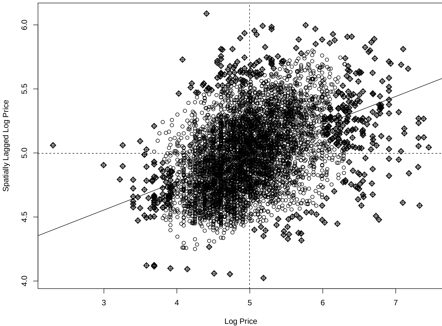
Moran Scatterplot – Spatial Clustering
