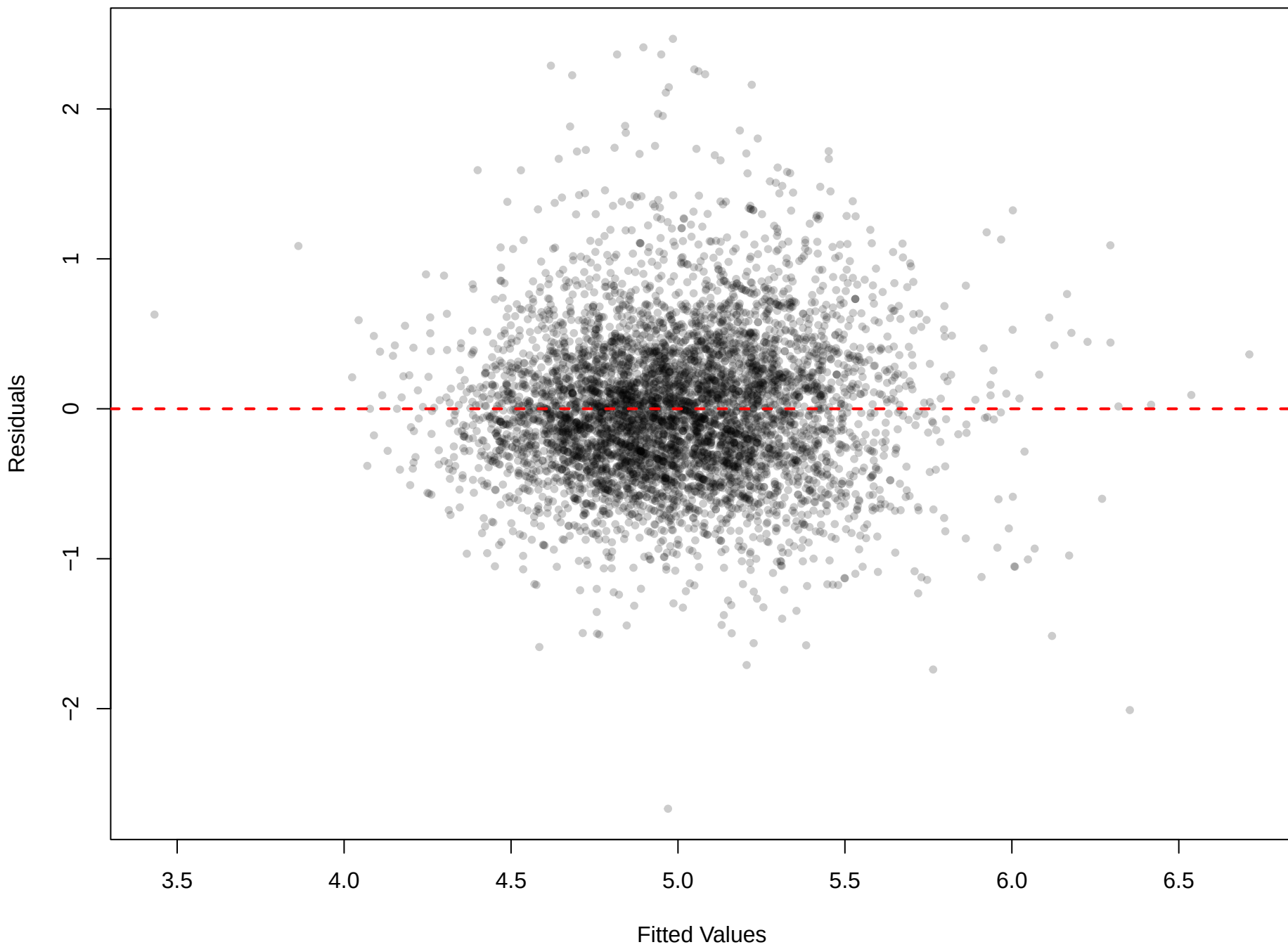
Residuals vs Fitted (Winning Model: SDM )
