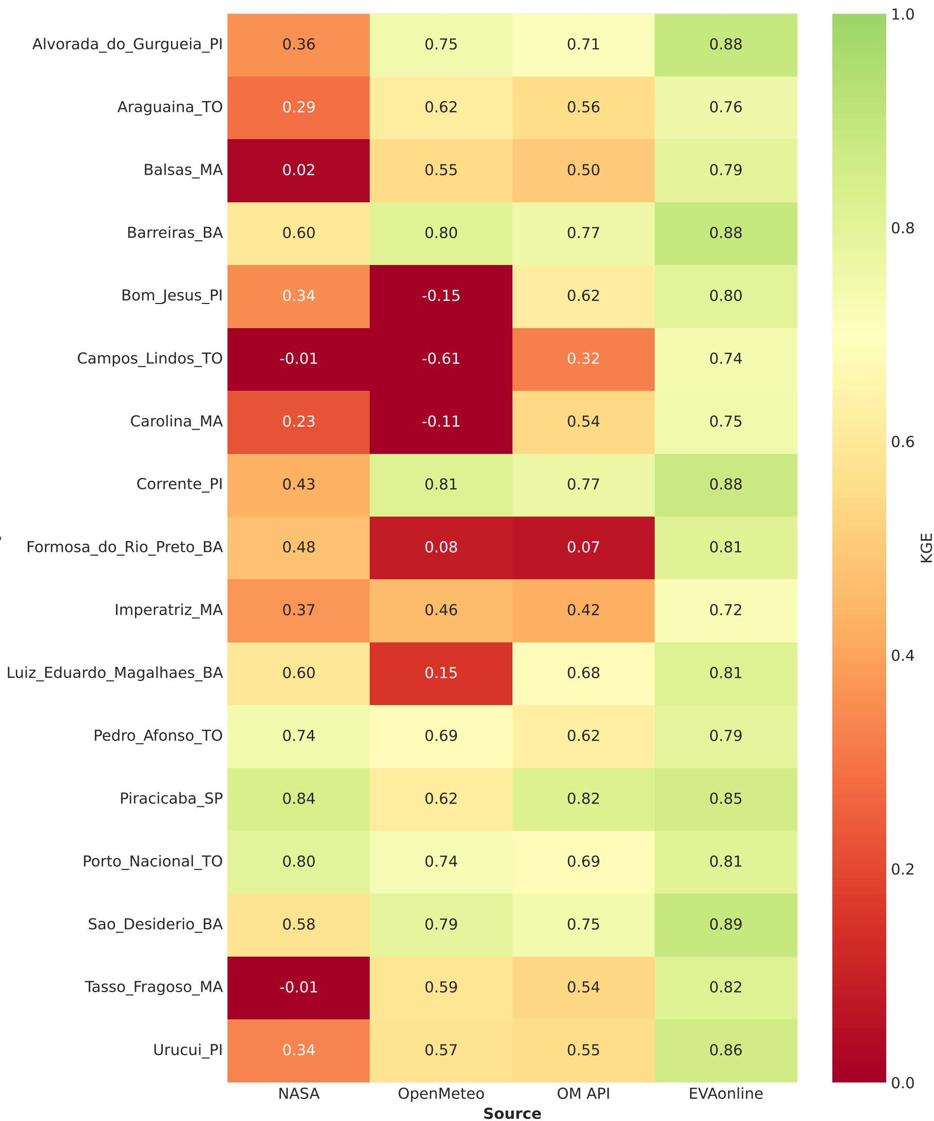
KGE (Kling-Gupta Efficiency) by City and Source
