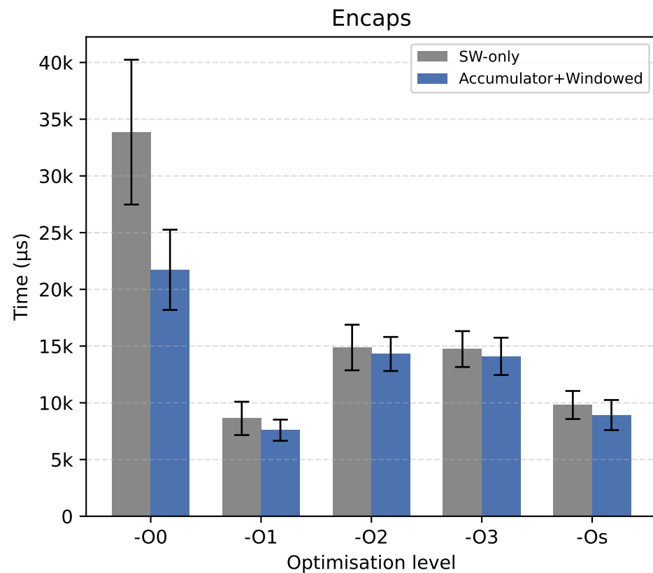
Wall-clock time: SW-only vs accumulator and windowed assembly (100 runs, error bars = 1 std dev)
