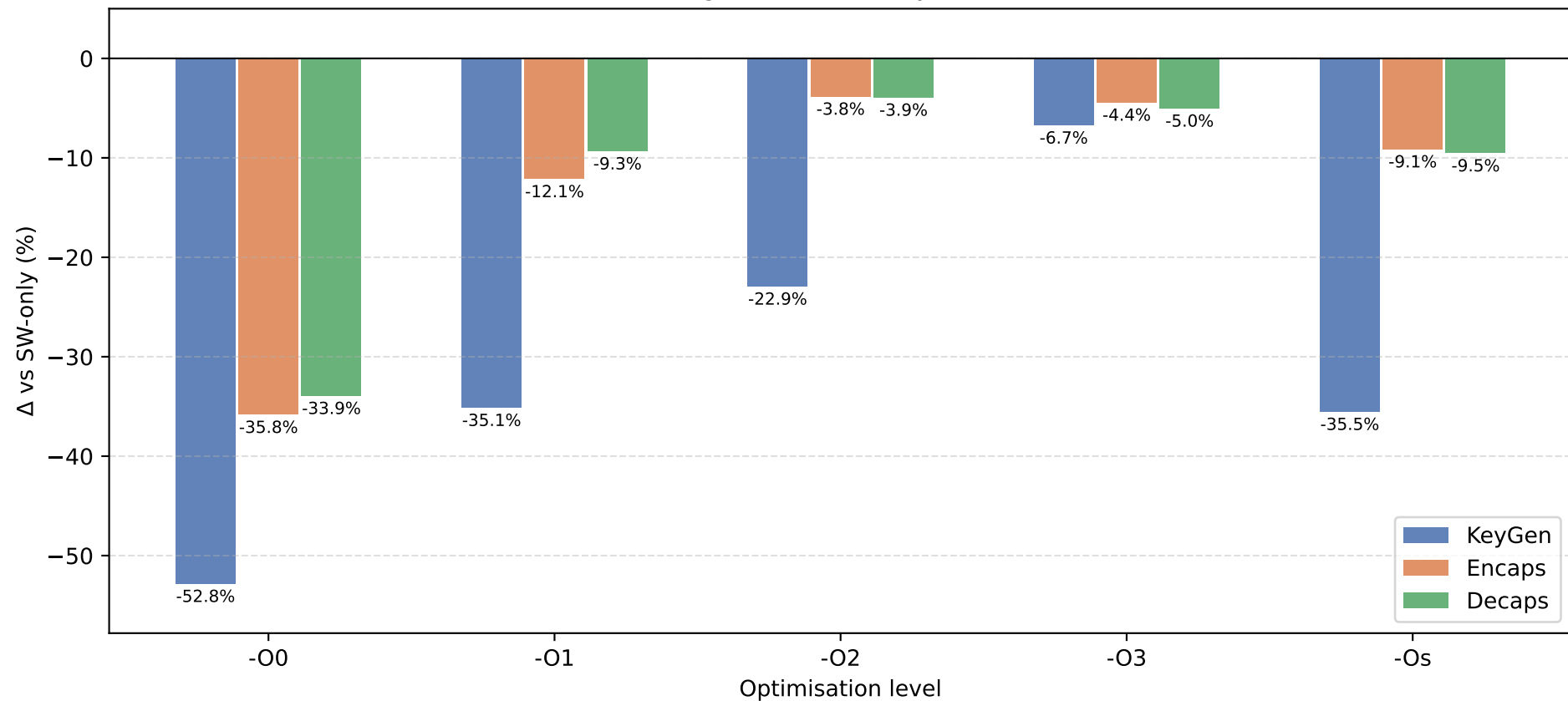
Accumulator and windowed assembly improvement over SW-only (negative = assembly faster)
