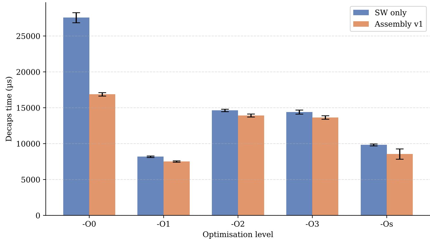
Decaps: SW-only vs Assembly v1 under QEMU (100 runs, error bars = 1 std dev)
