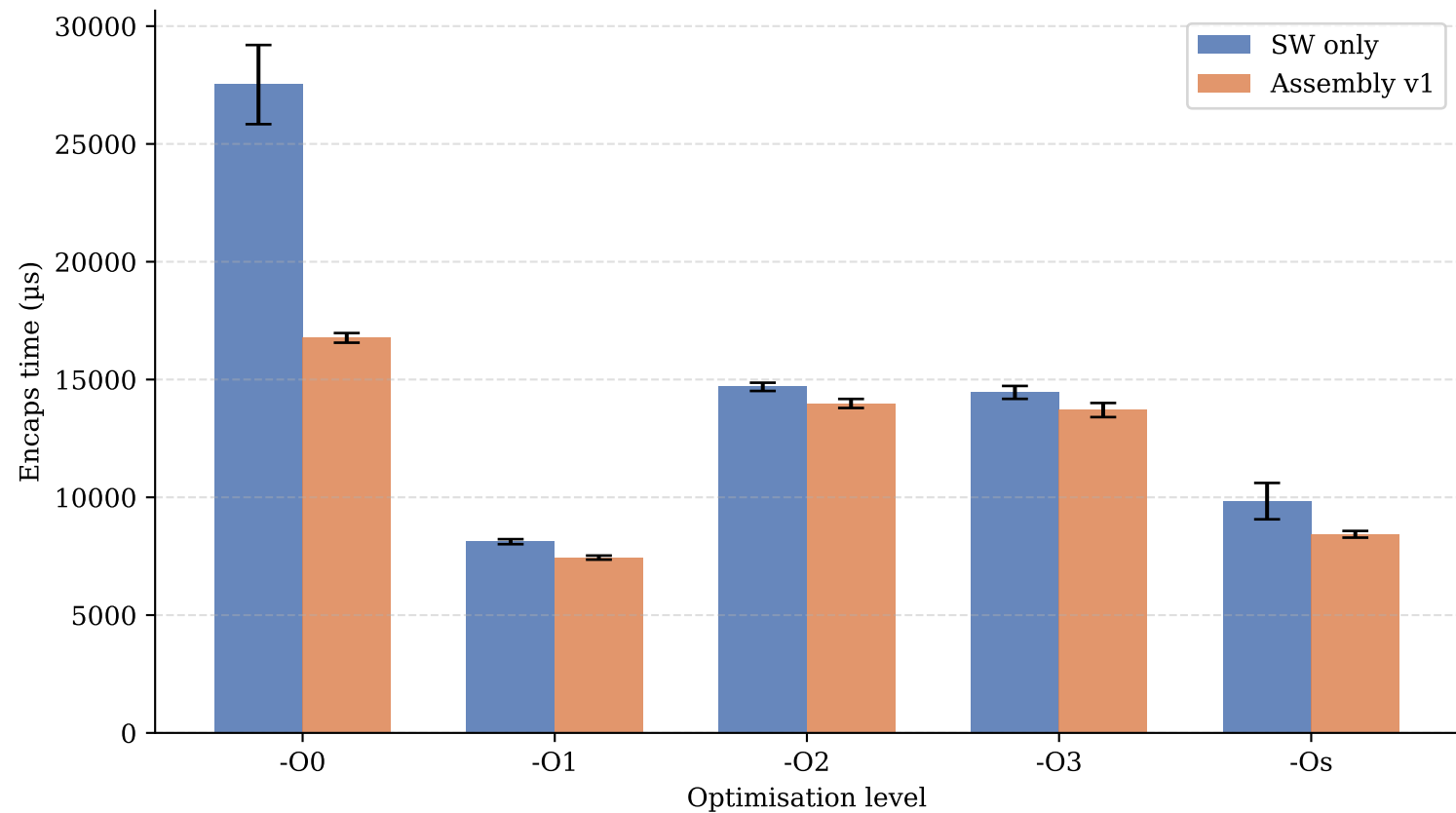
Encaps: SW-only vs Assembly v1 under QEMU (100 runs, error bars = 1 std dev)
