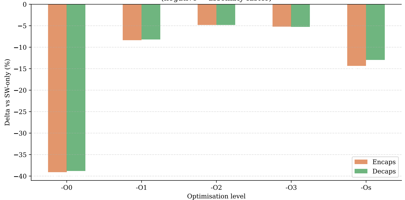
Encaps and Decaps improvement: Assembly v3 over SW-only baseline (negative = assembly faster)
