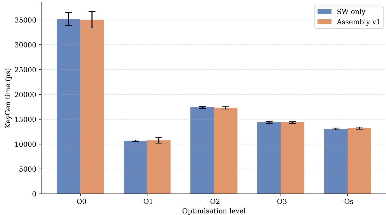
KeyGen: SW-only vs Assembly v1 under QEMU (100 runs, error bars = 1 std dev)
